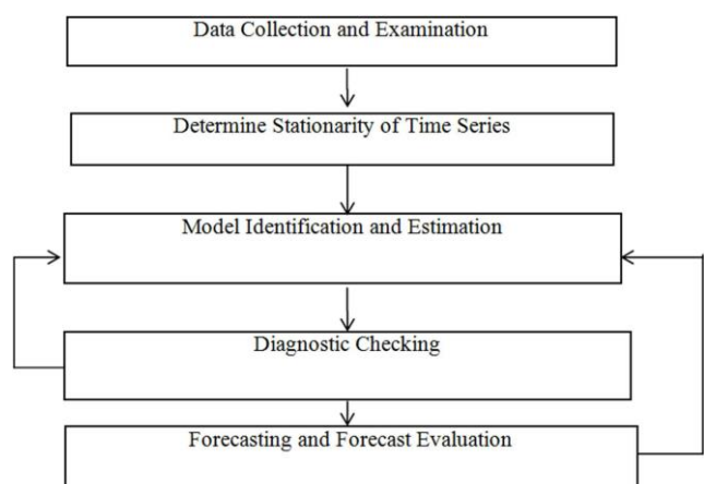
Figure 1. ARIMA forecasting procedure.
