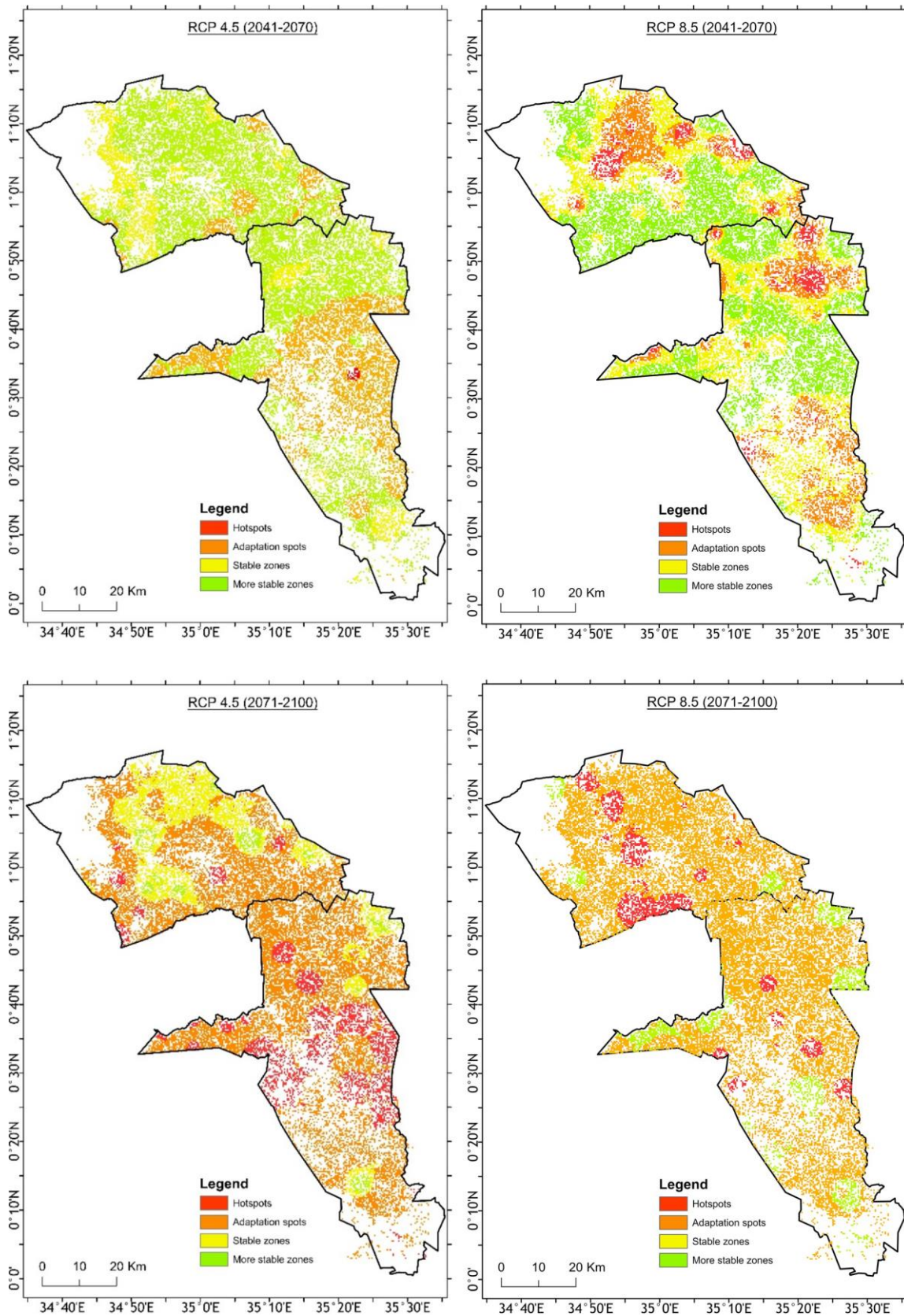
Fig. 3 Characterization of impact spots and stable maize yield zones for the mid-century period (2041–2070) and end-of-century period (2071–2100) under a RCP 4.5 and b RCP 8.5
