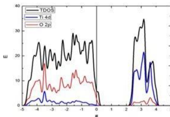
Figure 5: TDOS and PDOS of Ca doped Rutile
