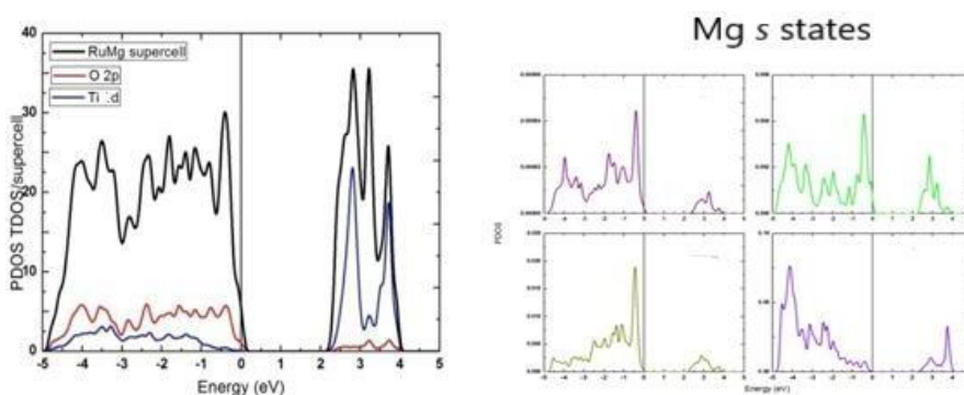
Figure 4: TDOS and PDOS Mg doped Rutile
