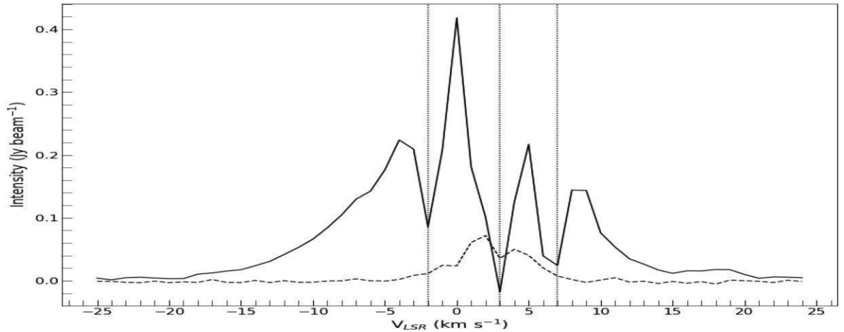
Figure 9. ^{12}\text{CO} (solid lines) and \text{CH}_3\text{OH} (dashed lines) spectra (of G188.95+0.89 extracted with an ellipse of size \sim 4 \text{ arcsec} centred on MM2). The vertical lines indicate the observed absorption features in ^{12}\text{CO} line. The multiple absorption features in the ^{12}\text{CO} emission and the double peak feature in the \text{CH}_3\text{OH} point to multiplicity (or at least binary) of driving sources in MM2. Band 7 ALMA dust continuum detected 2 cores in MM2.
