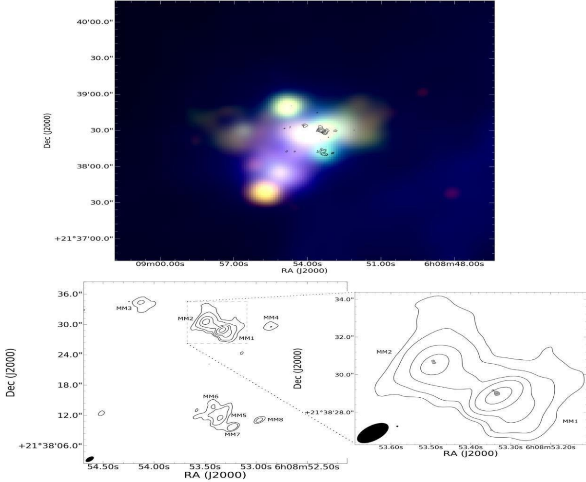
Figure 5. (Top) Composite three-colour WISE image of G188.95+0.89. WISE band 1 (3.4 μm), 2, (4.6 μm), and 3 (12 μm) are represented red, green, and blue. (bottom) ALMA band 6 (black contour, levels = [2, 4, 10, 20, 50] mJy beam -1 ) and in the zoom-in, band 7 (grey contour, levels = [2, 4, 20, 60, 80] mJy beam -1 ) dust continuum emission of G188.95+0.89. The filled ellipses on the bottom left-hand corner beams of the band 6 (larger ellipse) and band 7 (smaller ellipse). The open circle near MM1 peak indicates the position of the periodic 6.7-GHz CH 3 OH masers.
