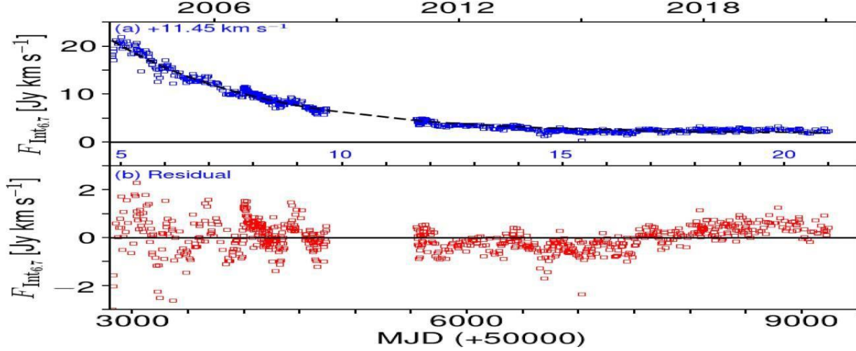
Figure 4. (a) Time series plot of F_{\text{Int } 6.7} for the v_{\text{LSR}} = +11.45 \text{ km s}^{-1} feature. The fitted
