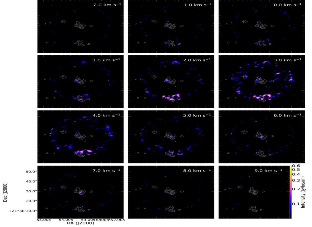
Figure 6. \text{CH}_3\text{OH } 4(2,2)\text{-}3(1,2) thermal line channel map with dust continuum overlaid (black contour, levels = [0.002, 0.004, 0.02, 0.06, 0.08] \text{Jy beam}^{-1} ) dust continuum emission of G188.95+0.89. The colour scale is the intensity in \text{Jy beam}^{-1} .
