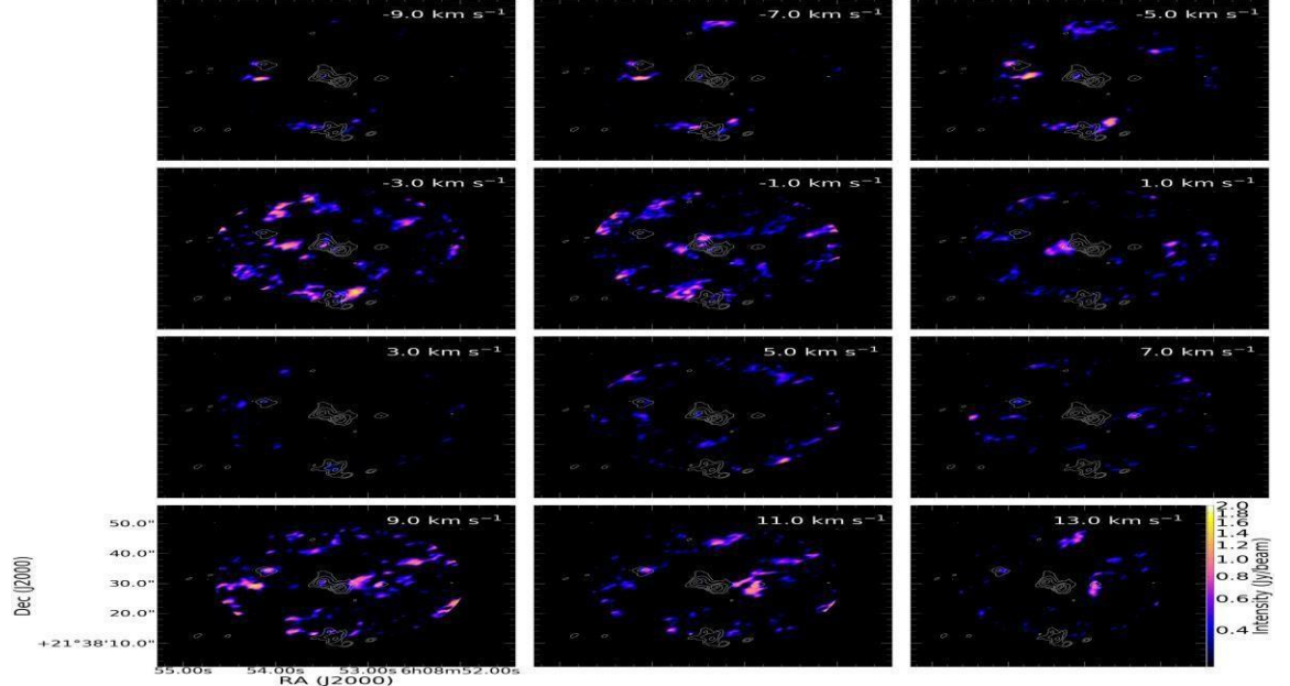
Figure 8. ^{12}\text{CO} ( J = 2 - 1 ) channel map with dust continuum overlaid (black contour, levels = [0.002, 0.004, 0.02, 0.06, 0.08] \text{Jy beam}^{-1} ) dust continuum emission of G188.95 + 0.89. The color scale is the intensity in \text{Jy beam}^{-1} .
