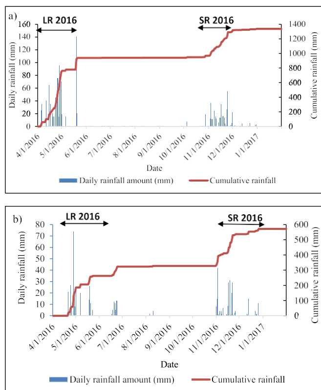
Fig. 1. Daily and cumulative rainfall during the experimental period in Chuka (a) and Kandara (b) sites.
