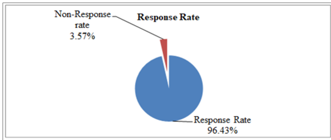
Figure 1: Response rate
