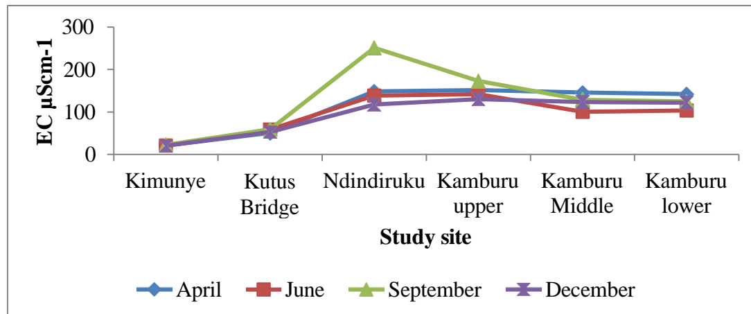
Figure 3: Spatial and temporal variations in EC values along the study site
