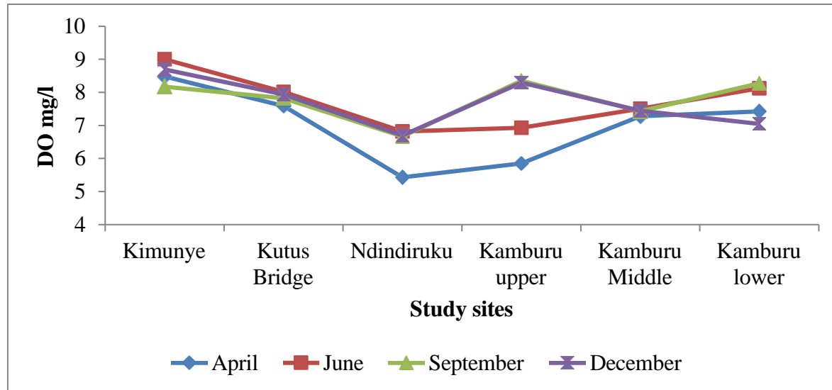
Figure 2: Spatial and temporal changes in DO values along the study site
