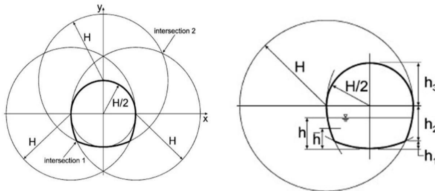
Fig. 1. Cross-section of a horseshoe channel
