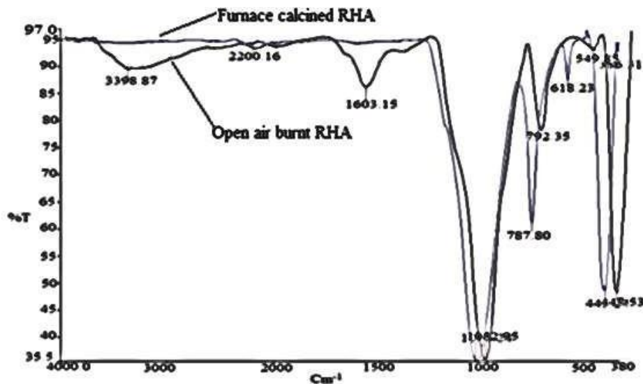
Figure 5. FTIR Spectra of oRHA and fRHA.
