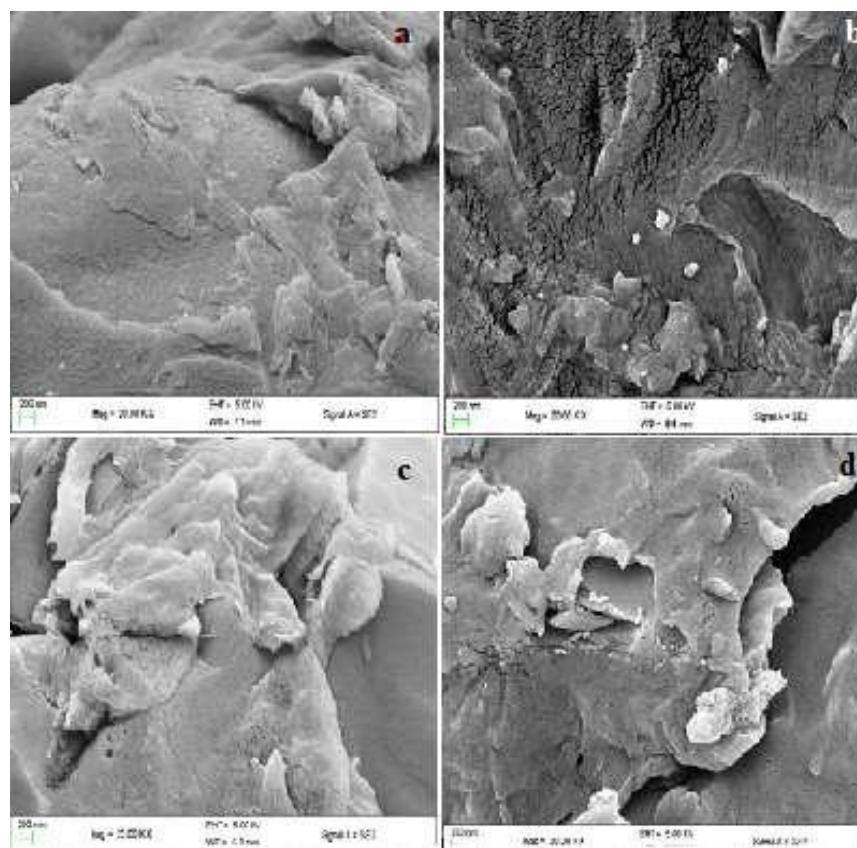
Figure 12. SEM micrographs for 50% RHA-HDPE samples (magnification 20000x) for oRHA with a. pure HDPE, b. recycled HDPE and for fRHA c. Pure HDPE and d. recycled HDPE.
