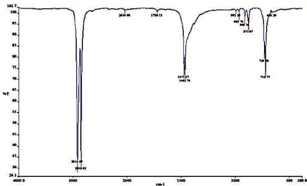
Figure 3. FTIR Spectra of pure HDPE pellets.
