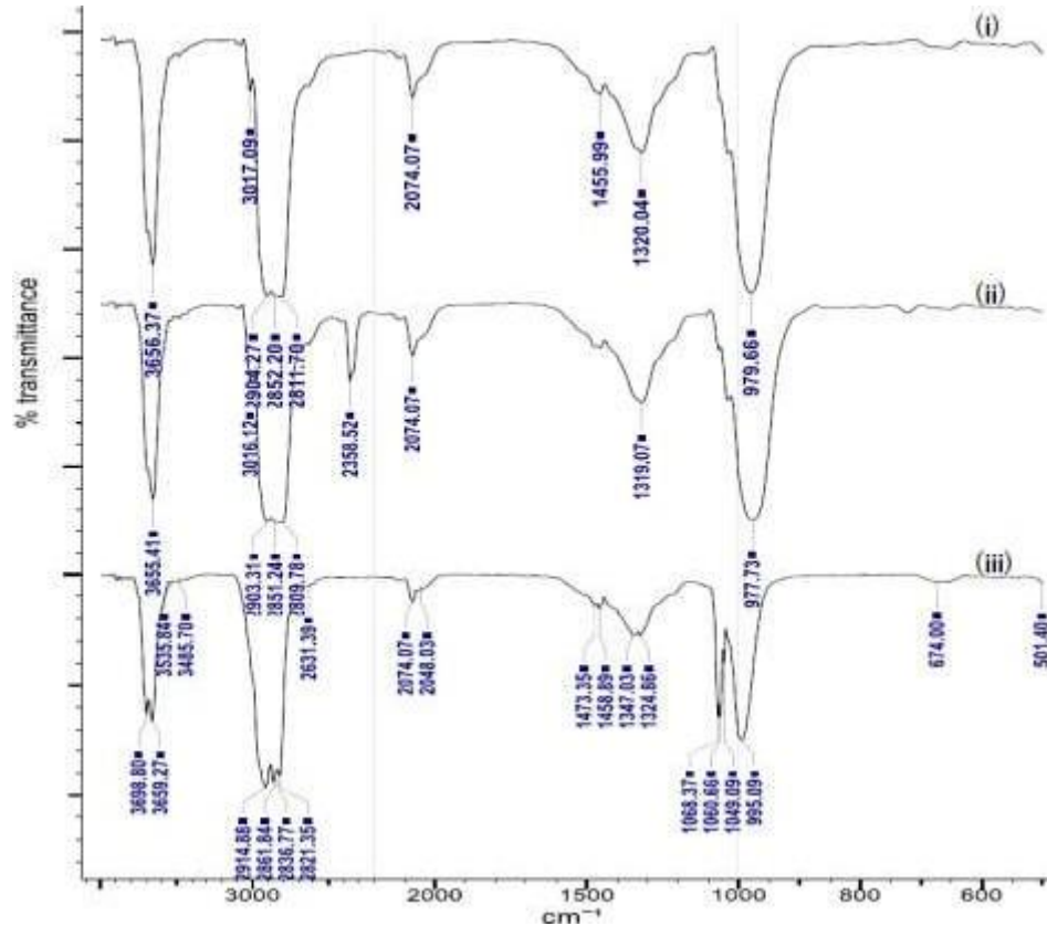
Figure 9. FTIR spectra for oRHA-MA-HDPE (recycled) composites (i) 5 % oRHA (ii) 10% oRHA and (iii) 35 % oRHA.
