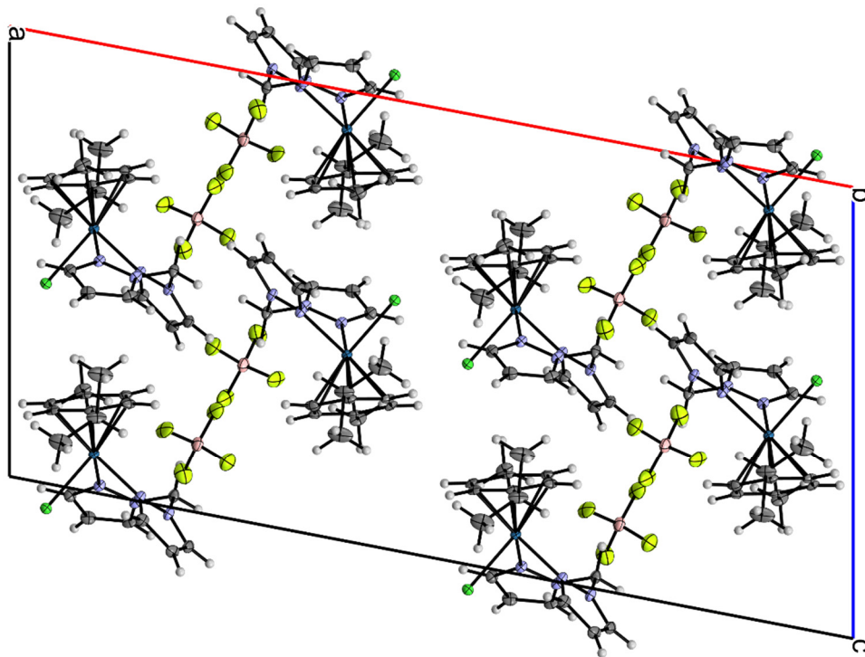
Figure 2. The unit cell and the packing of 1 ( C_{17}H_{22}BClF_4N_4Os ).
